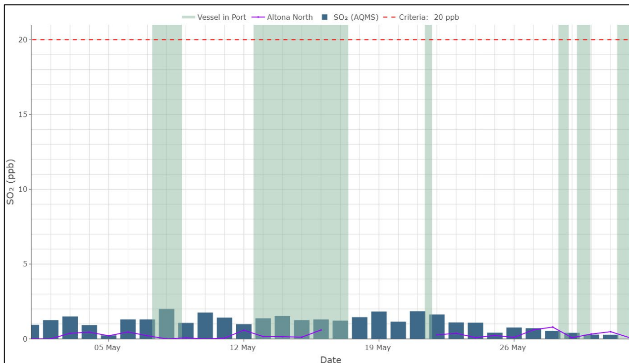
Figure 6 24-hour average SO 2 concentrations (ppb) at Station Pier and local EPA Station (May 2024) (criteria: 20 ppb)
