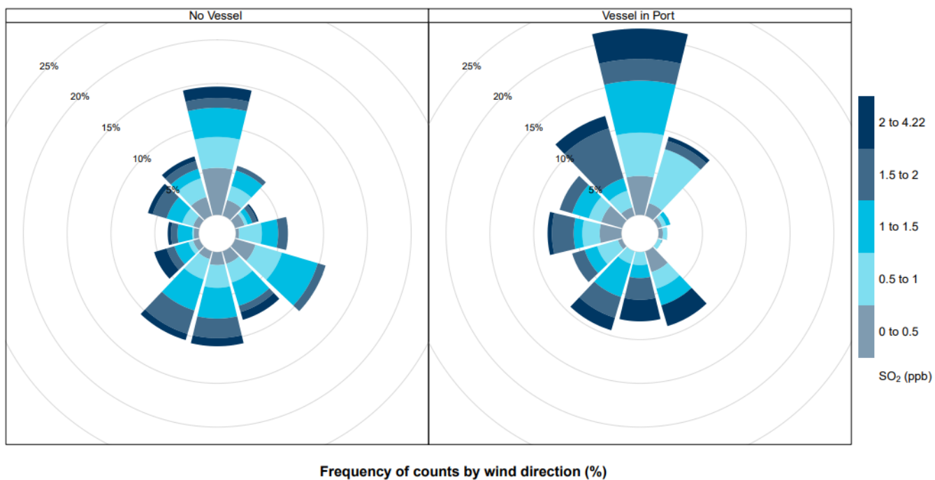
Figure B.17 Hourly average SO 2 concentration (ppb) pollution roses (May 2024)
