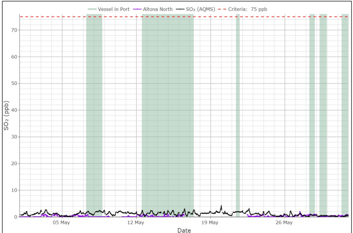
Figure B.22 Hourly average SO 2 concentrations (ppb) at Station Pier and local EPA stations (May 2024) (criteria: 75 ppb)
