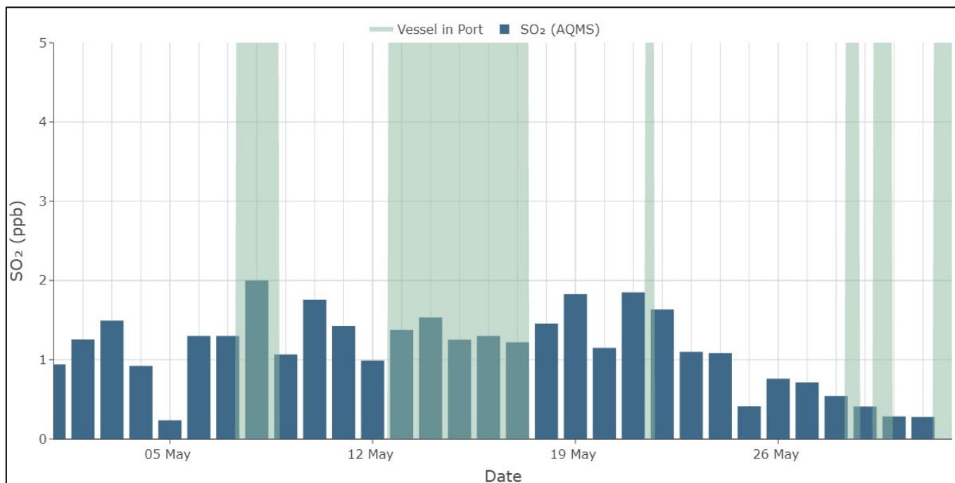
Figure B.18 24-hour average SO 2 concentrations (ppb) at Station Pier (May 2024) (criteria: 20 ppb)
