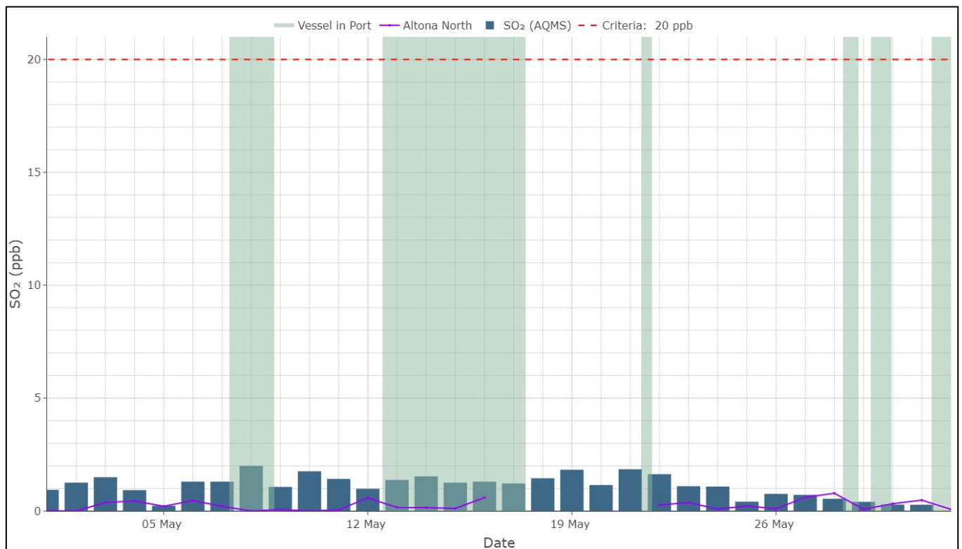
Figure B.23 24-hour average SO 2 concentrations (ppb) at Station Pier and local EPA Station (May 2024) (criteria: 20 ppb)
