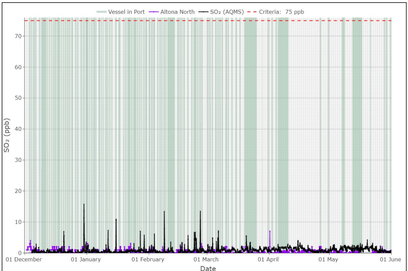
Figure C.7 Hourly average SO 2 concentrations (ppb) at Station Pier and local EPA Station (December 2023 - May 2024) (criteria: 75 ppb)
