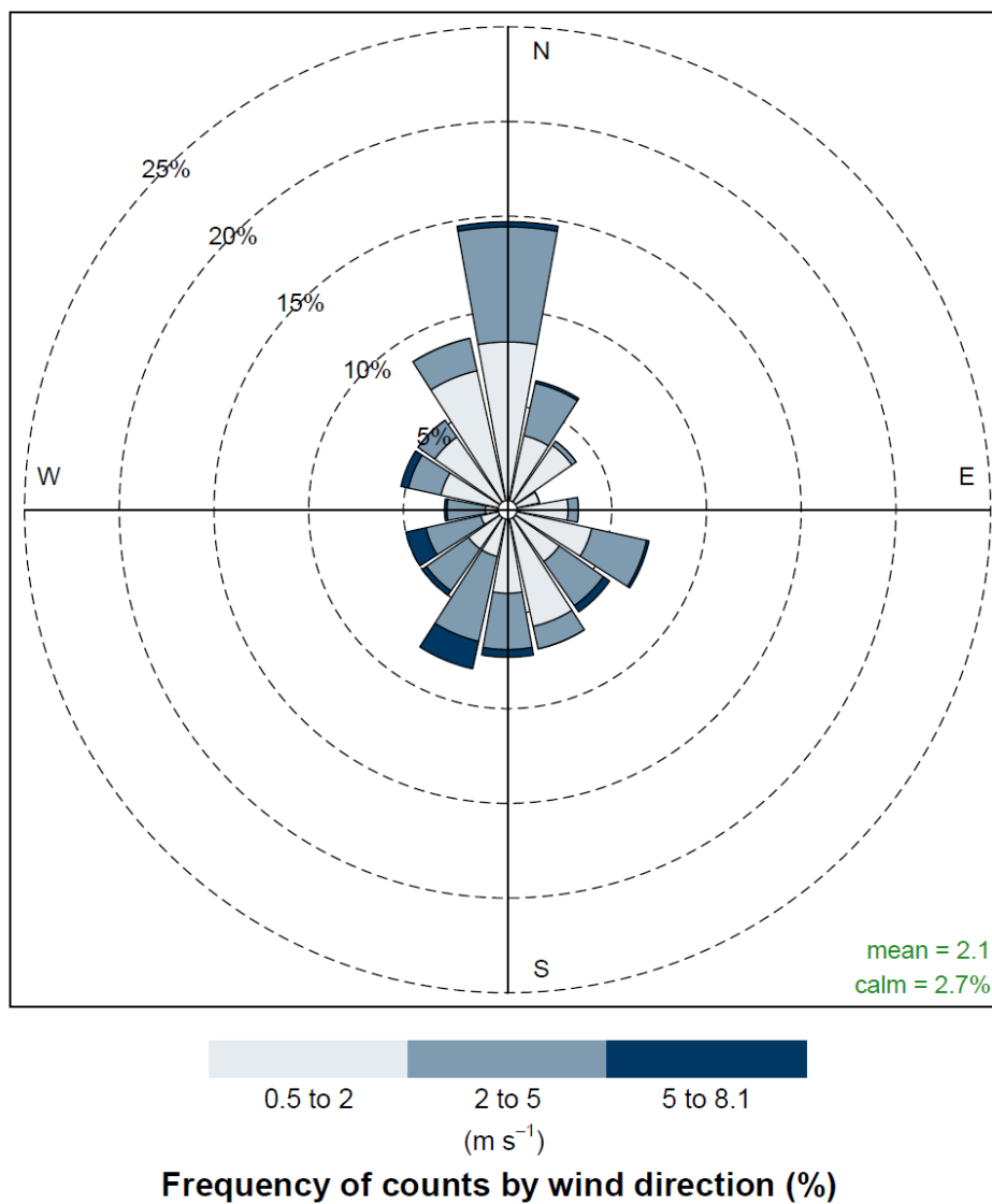
Figure B.2 May 2024 windrose at Station Pier
