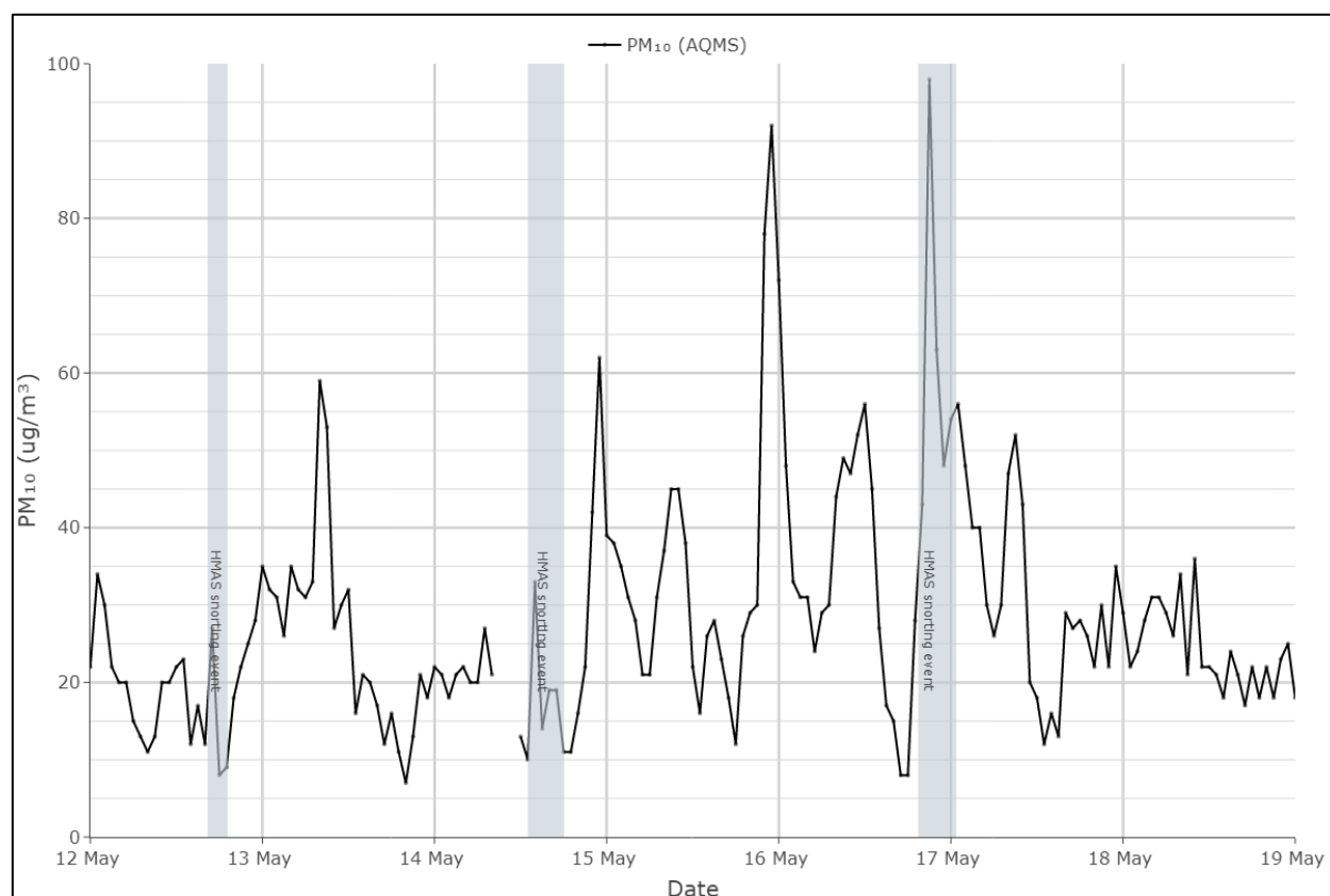
Figure B.26 Hourly average PM_{10} concentrations ( \mu g/m^3 ) at Station Pier during 'snorting' events
