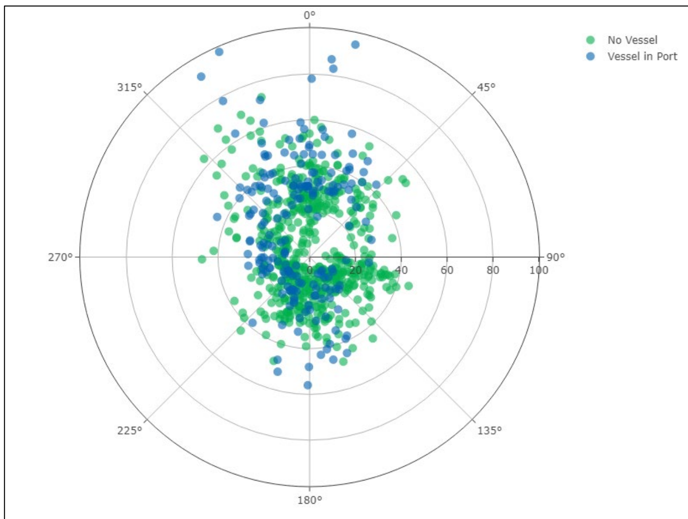
Figure B.7 Hourly average PM_{10} concentration ( \mu g/m^3 ) by wind direction (May 2024)
