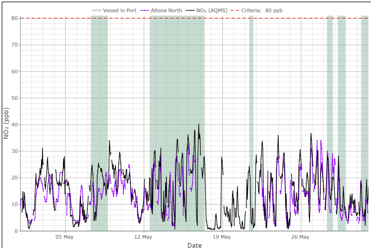
Figure 4 Hourly average NO 2 concentrations (ppb) at Station Pier and local EPA stations (May 2024) (criteria: 80 ppb)
