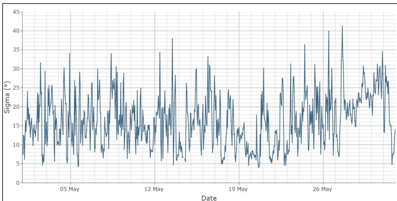
Figure B.5 May 2024 sigma observations at Station Pier
