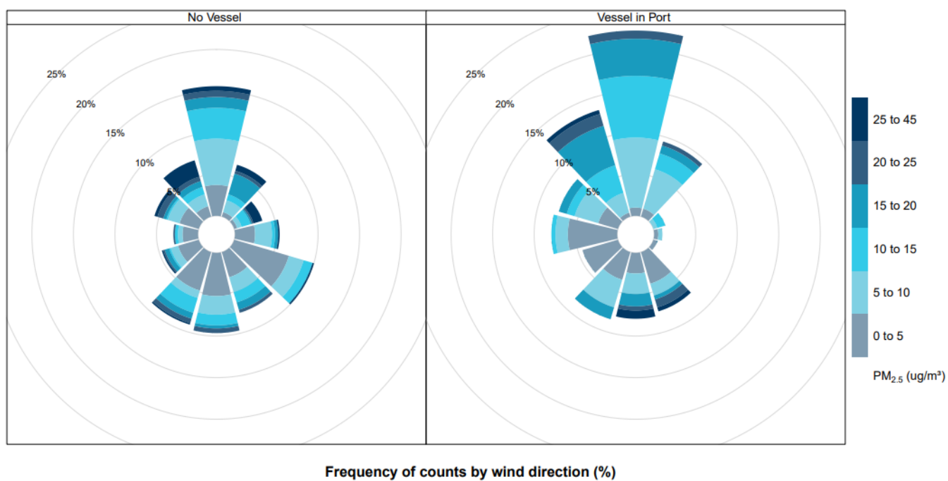
Figure B.11 Hourly average PM_{2.5} concentration ( \mu\text{g}/\text{m}^3 ) pollution roses (May 2024)
