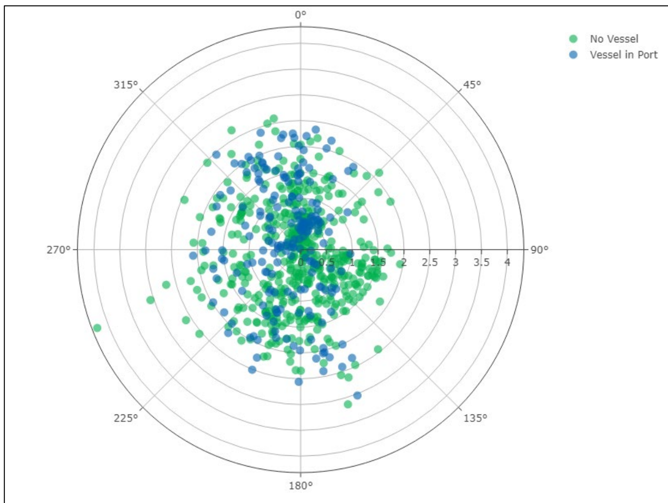
Figure B.16 Hourly average SO 2 concentration (ppb) by wind direction (May 2024)
