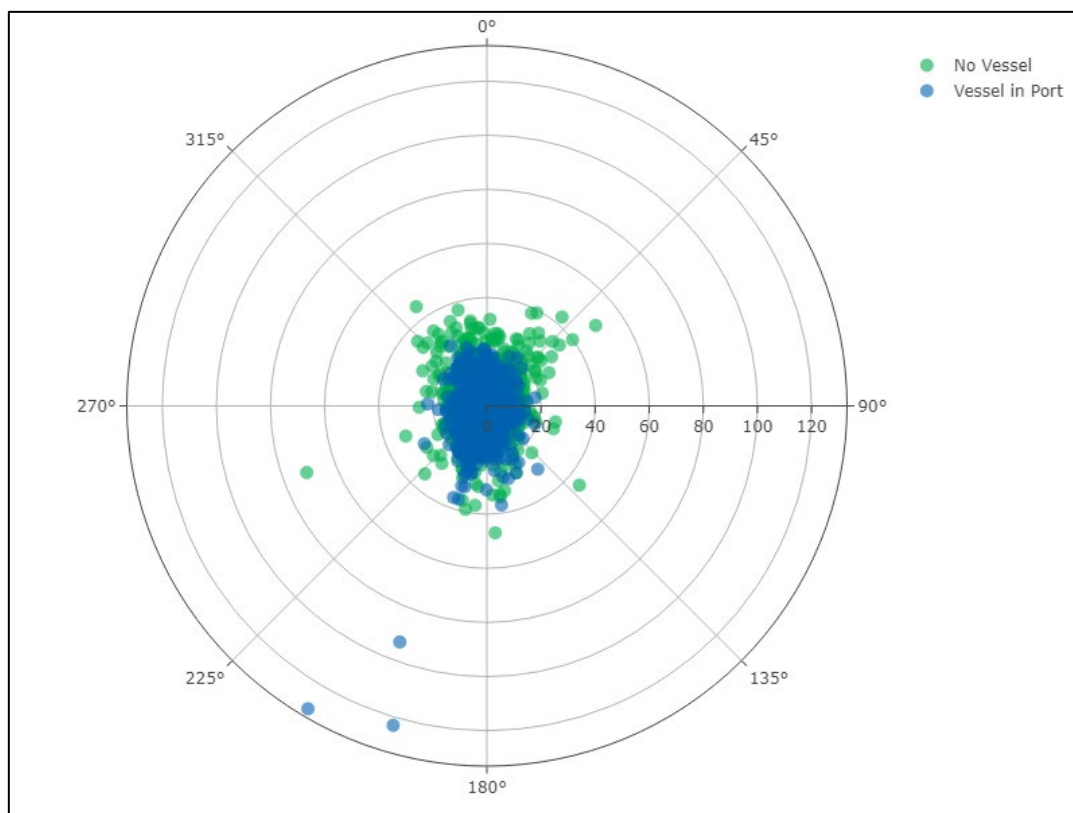
Figure C.4 Hourly average PM_{2.5} concentration ( \mu\text{g}/\text{m}^3 ) by wind direction (December 2023 - May 2024)
