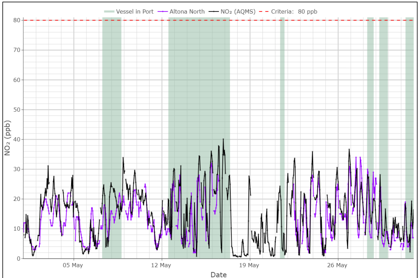
Figure B.21 Hourly average NO 2 concentrations (ppb) at Station Pier and local EPA Station (May 2024) (criteria: 80 ppb)
