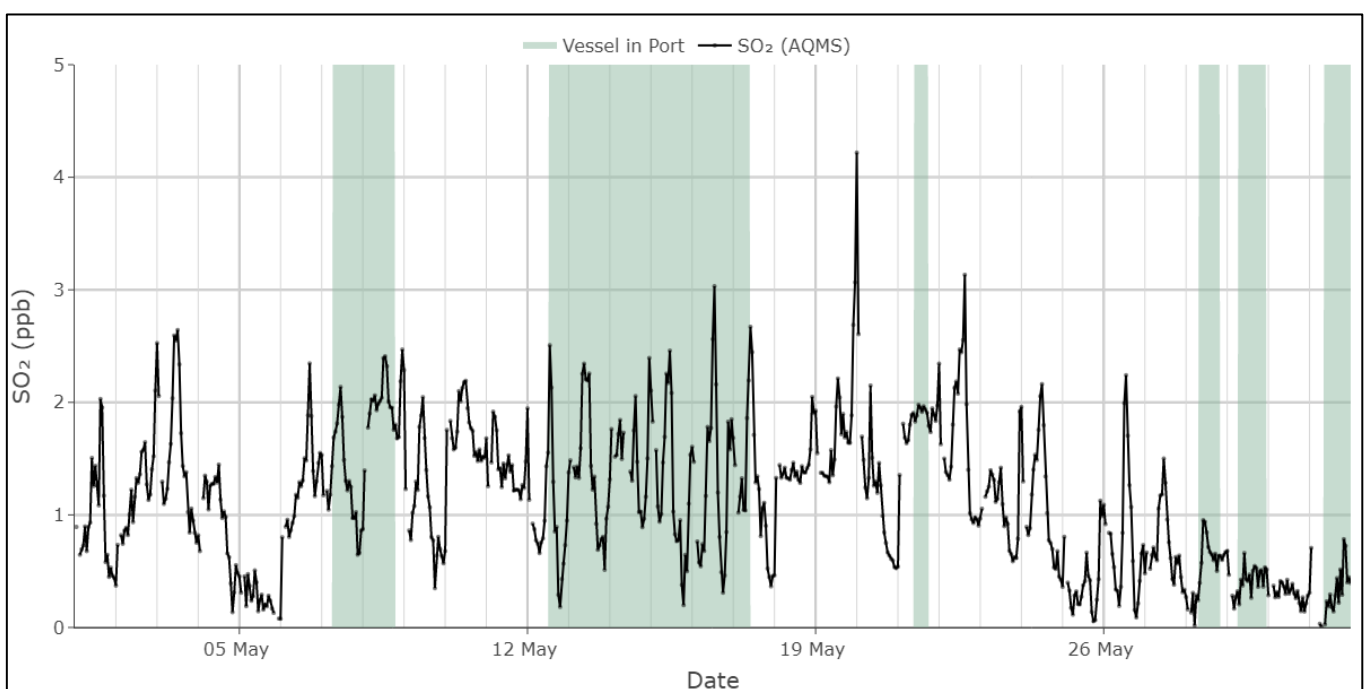
Figure B.15 Hourly average SO 2 concentrations (ppb) at Station Pier (May 2024) (criteria: 75 ppb)
