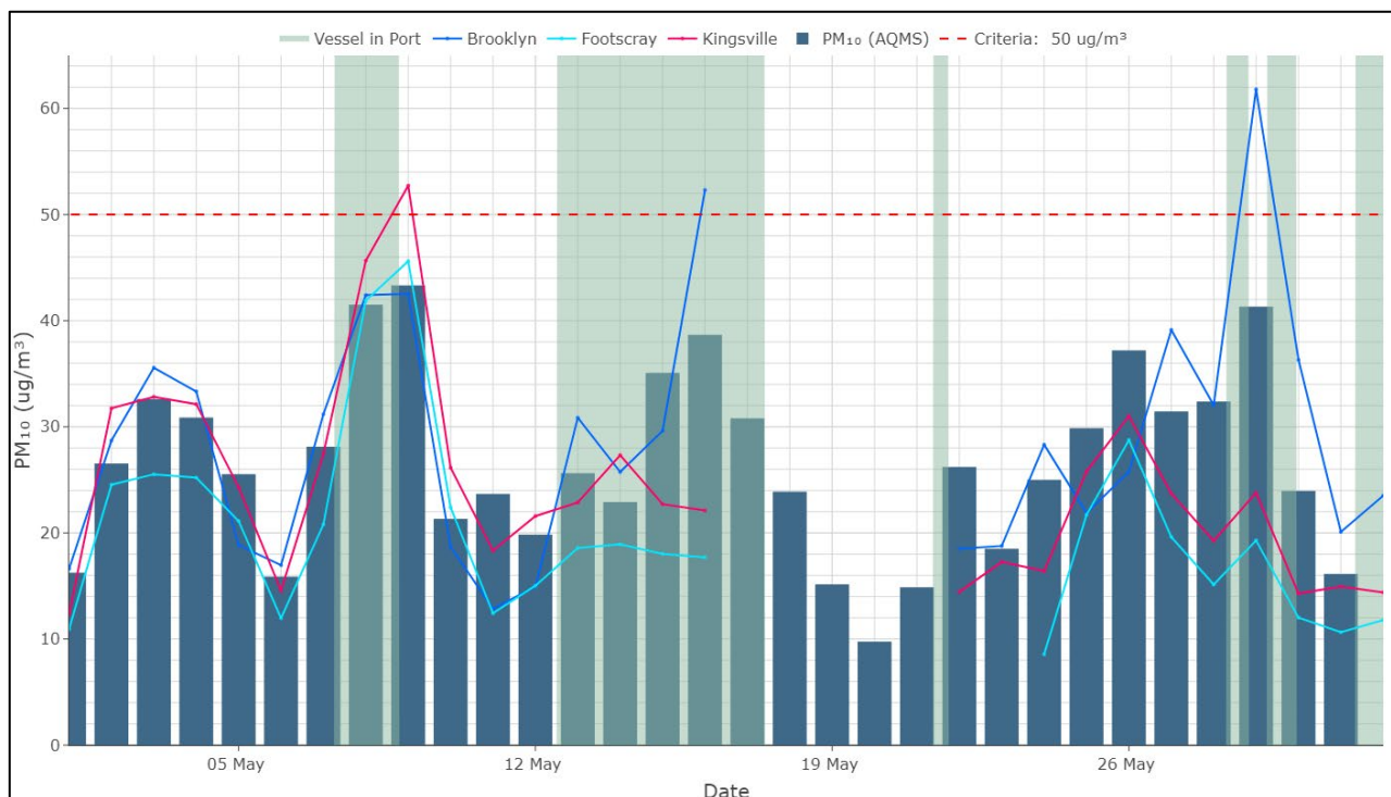
Figure 2 24-hour average PM 10 concentrations ( \mu\text{g}/\text{m}^3 ) at Station Pier and local EPA stations (May 2024) (criteria: 50 \mu\text{g}/\text{m}^3 )
