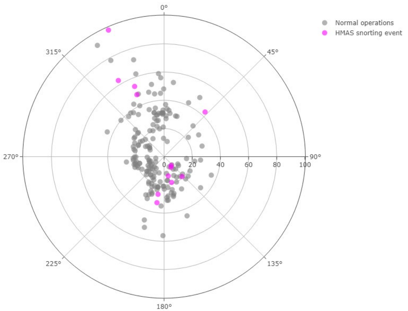
Figure B.27 Hourly average \text{PM}_{10} concentration ( \mu\text{g}/\text{m}^3 ) observed at AQMS between 12 and 19 May by wind direction (May 2024)
