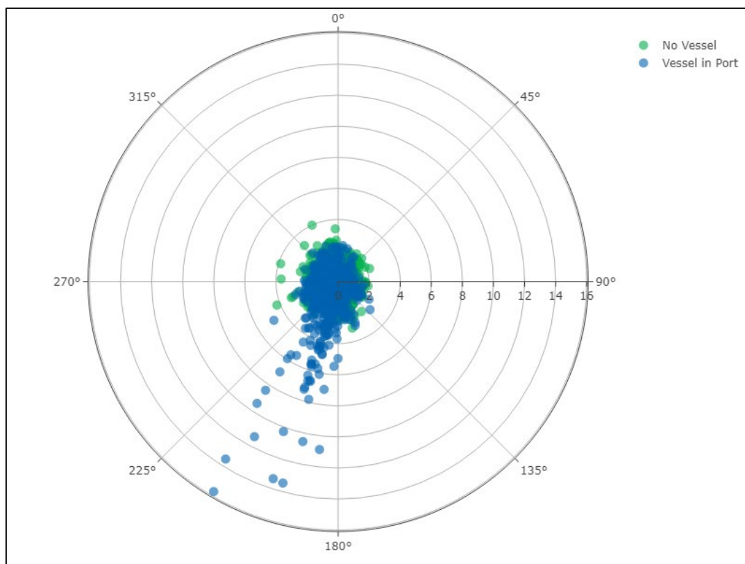
Figure C.8 Hourly average \text{SO}_2 concentration ( \mu\text{g}/\text{m}^3 ) by wind direction (December 2023 - May 2024)
