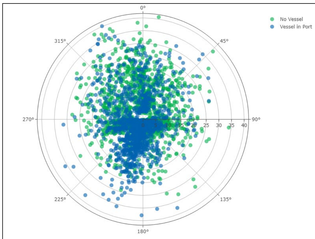
Figure C.6 Hourly average \text{NO}_2 concentration ( \mu\text{g}/\text{m}^3 ) by wind direction (December 2023 - May 2024)
