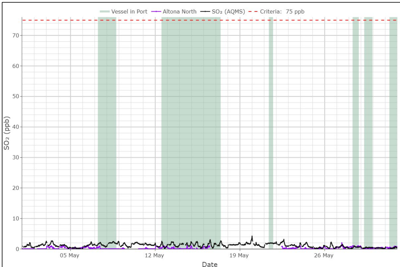
Figure 5 Hourly average SO 2 concentrations (ppb) at Station Pier and local EPA Station (May 2024) (criteria: 75 ppb)
