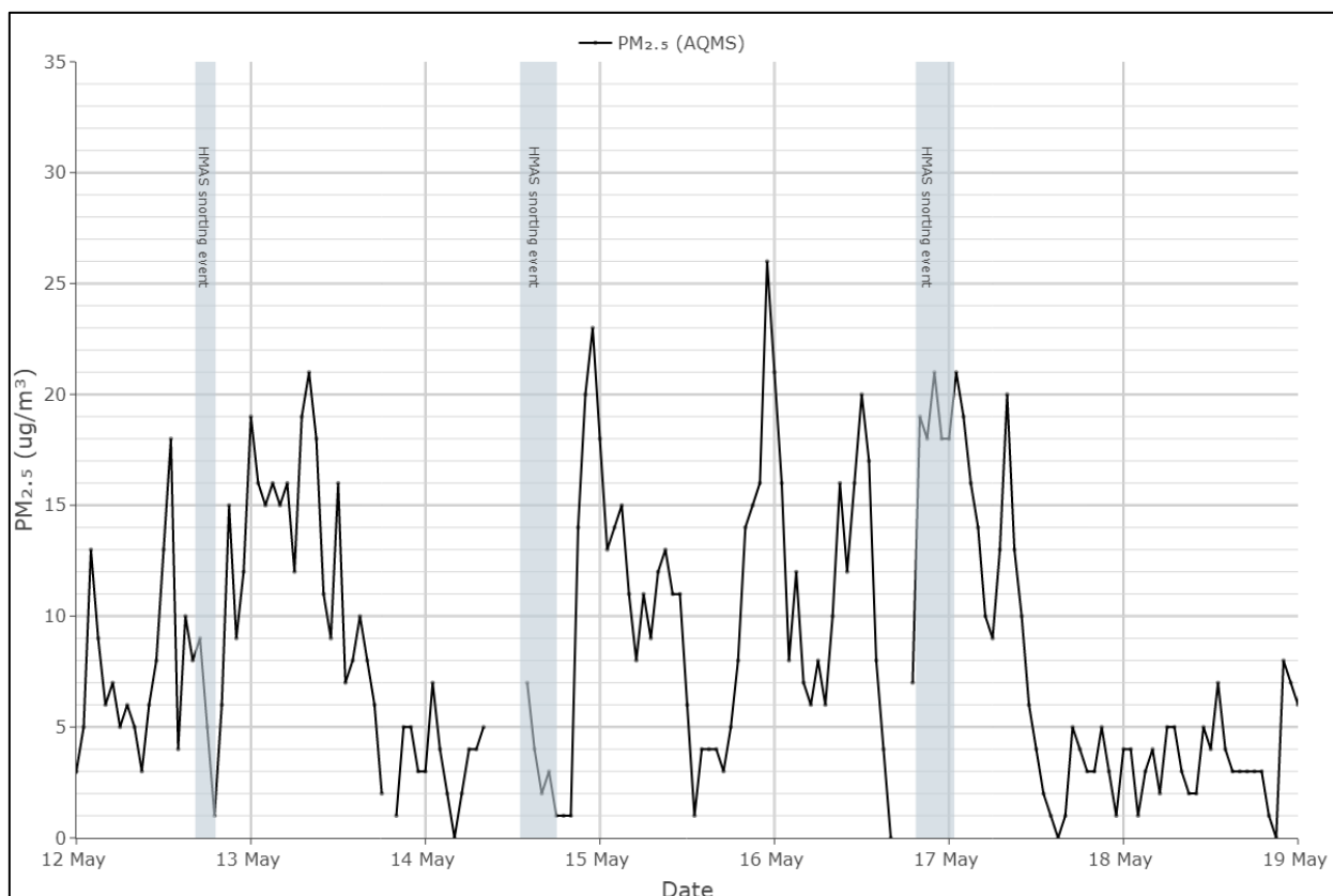
Figure B.28 Hourly average PM_{2.5} concentrations ( \mu g/m^3 ) at Station Pier during 'snorting' events
