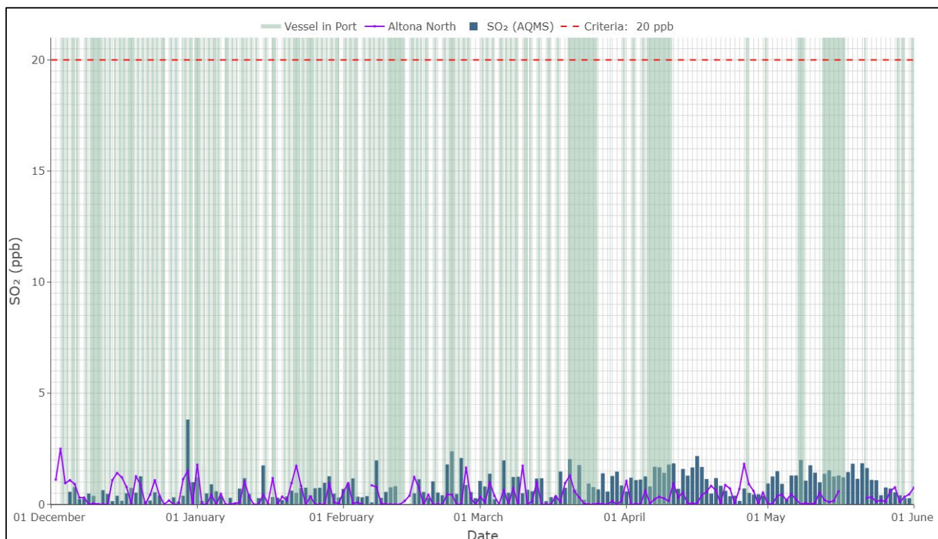
Figure C.9 24-hour average \text{SO}_2 concentrations ( \mu\text{g}/\text{m}^3 ) at Station Pier and local EPA Station (December 2023 - May 2024) (criteria: 20 \mu\text{g}/\text{m}^3 )
