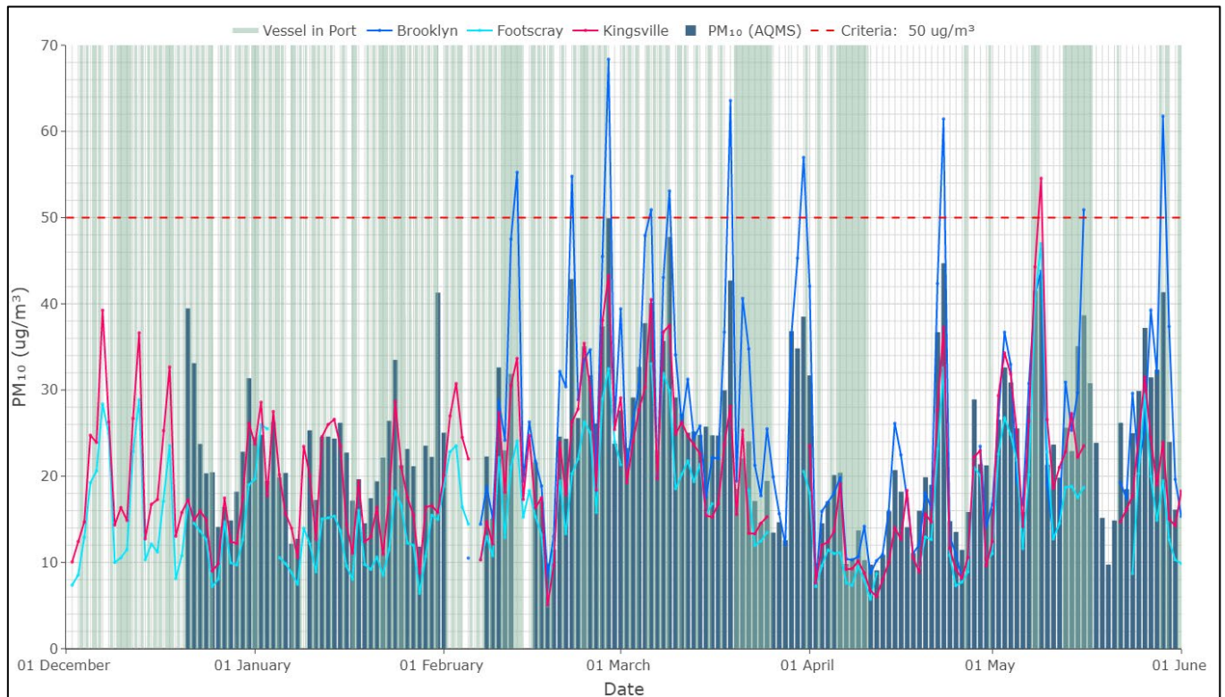
Figure C.1 24-hour average PM 10 concentrations (µg/m³) at Station Pier and local EPA stations (December 2023 - May 2024) (criteria: 50 µg/m³)
