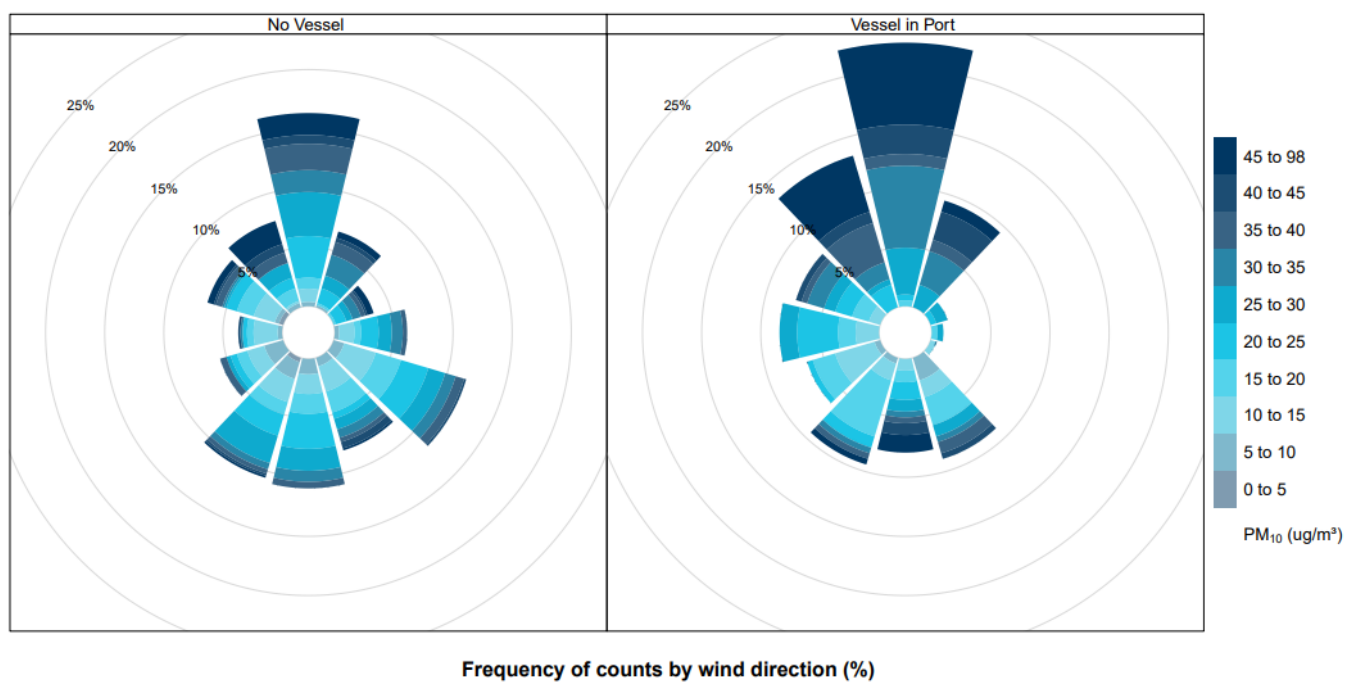
Figure B.8 Hourly average PM_{10} concentration ( \mu g/m^3 ) pollution roses (May 2024)
