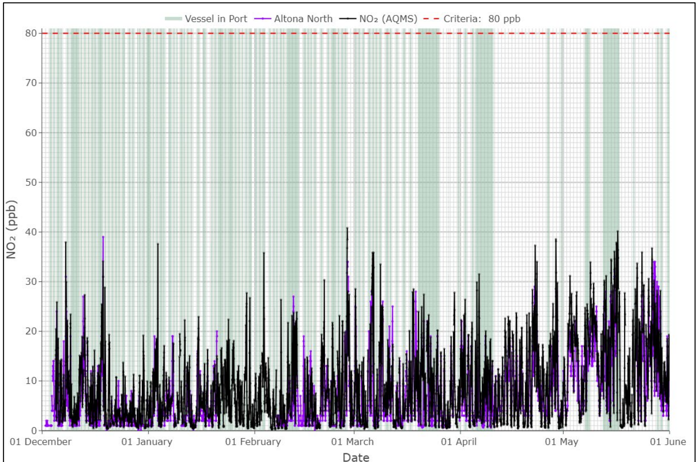
Figure C.5 Hourly average NO 2 concentrations (ppb) at Station Pier and local EPA stations (December 2023 - May 2024) (criteria: 80 ppb)
